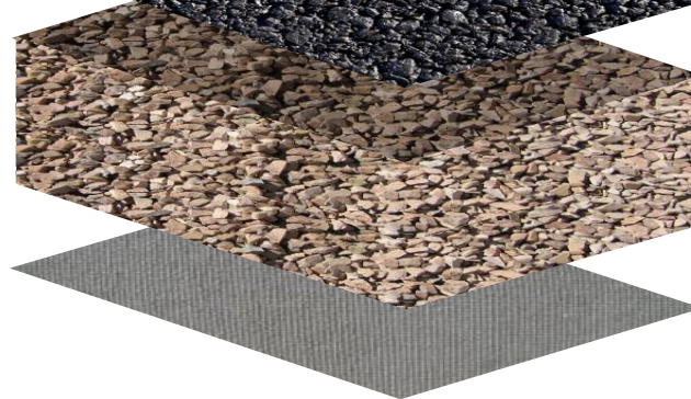
300-500mm MOT Type 3 Sub base Well compacted non frost susceptible Type 3 granular sub base to SHW clause 805 or 4/40mm, 4/20mm graded crushed concrete aggregate to EN 12620 or locally available secondary or recycled aggregate complying to the above specification
